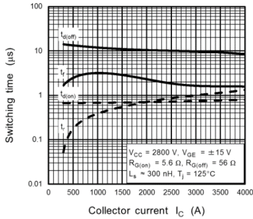
Figure 2.15 t_{d(on)} , t_r , t_{d(off)} , t_f - I_C Characteristics
