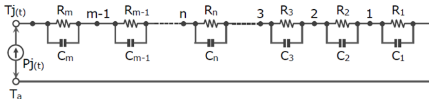
Figure 4.8 Thermal Impedance of Power Semiconductors
