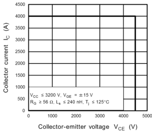
Figure 2.18 RBSOA Characteristics
