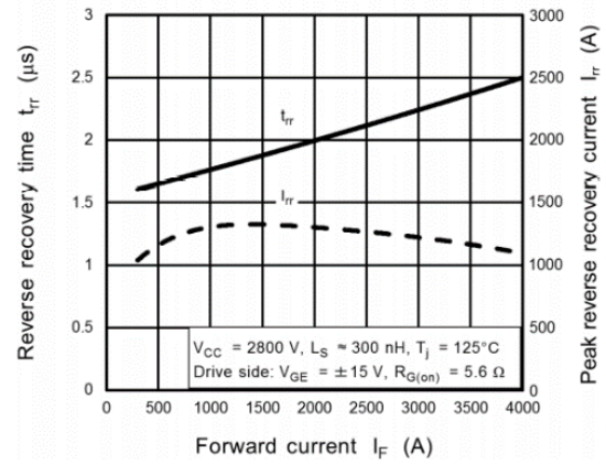
Figure 2.16 t_{rr} - I_{rr} - I_F Characteristics
