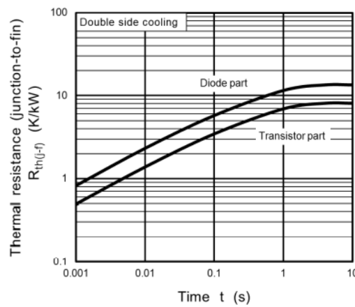
Figure 2.17 R_{th(j-f)-t} Characteristics
