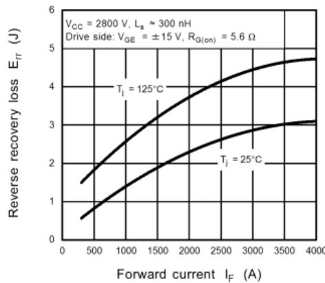
Figure 2.9 E rr -I F Characteristics
