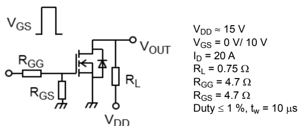
Fig. 6.2.1 Switching Time (Fig.)
