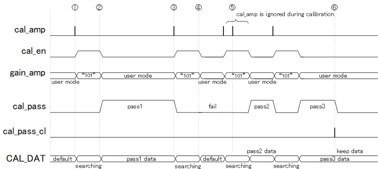
Fig. 7.3.2-2 Performing Offset Calibration
