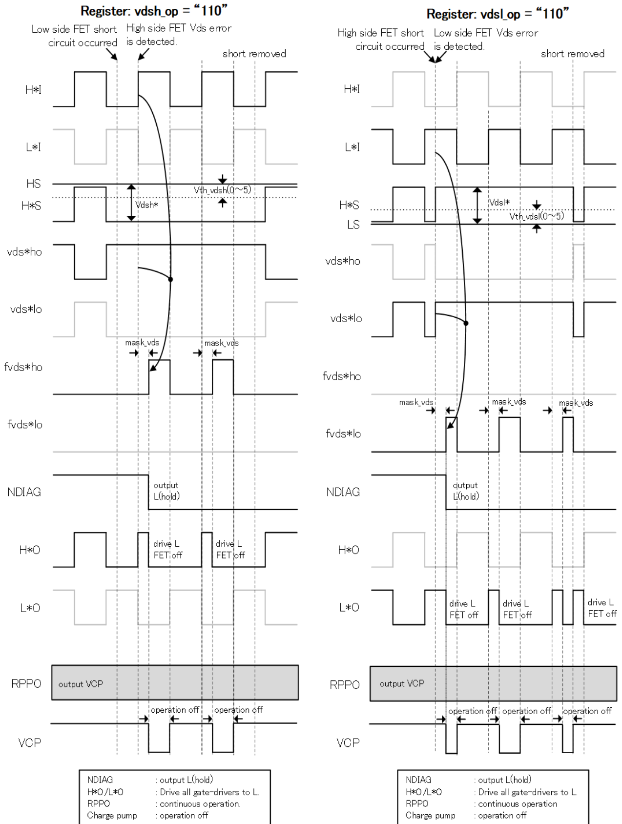
Fig. 7.6.7.8 Short-Circuit Detection Timing Chart (In the case of register: vds_lop = vds_op "110")
