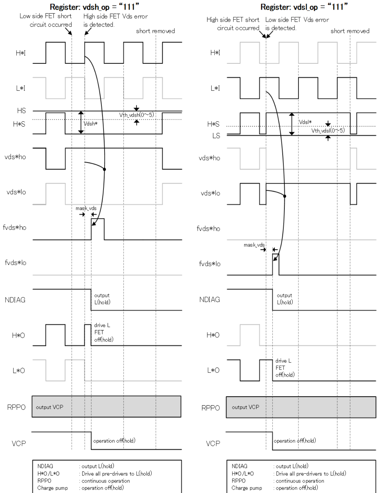
Fig. 7.6.7.9 Short-Circuit Detection Timing Chart (In the case of register: vds l _op = vds h _op "111")
