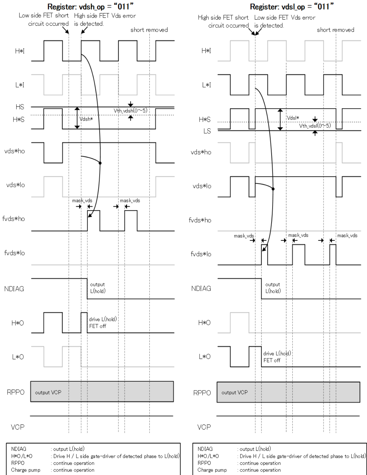
Fig. 7.6.7.5 Short-Circuit Detection Timing Chart (In the case of register: vds l _op = vds h _op "011")
