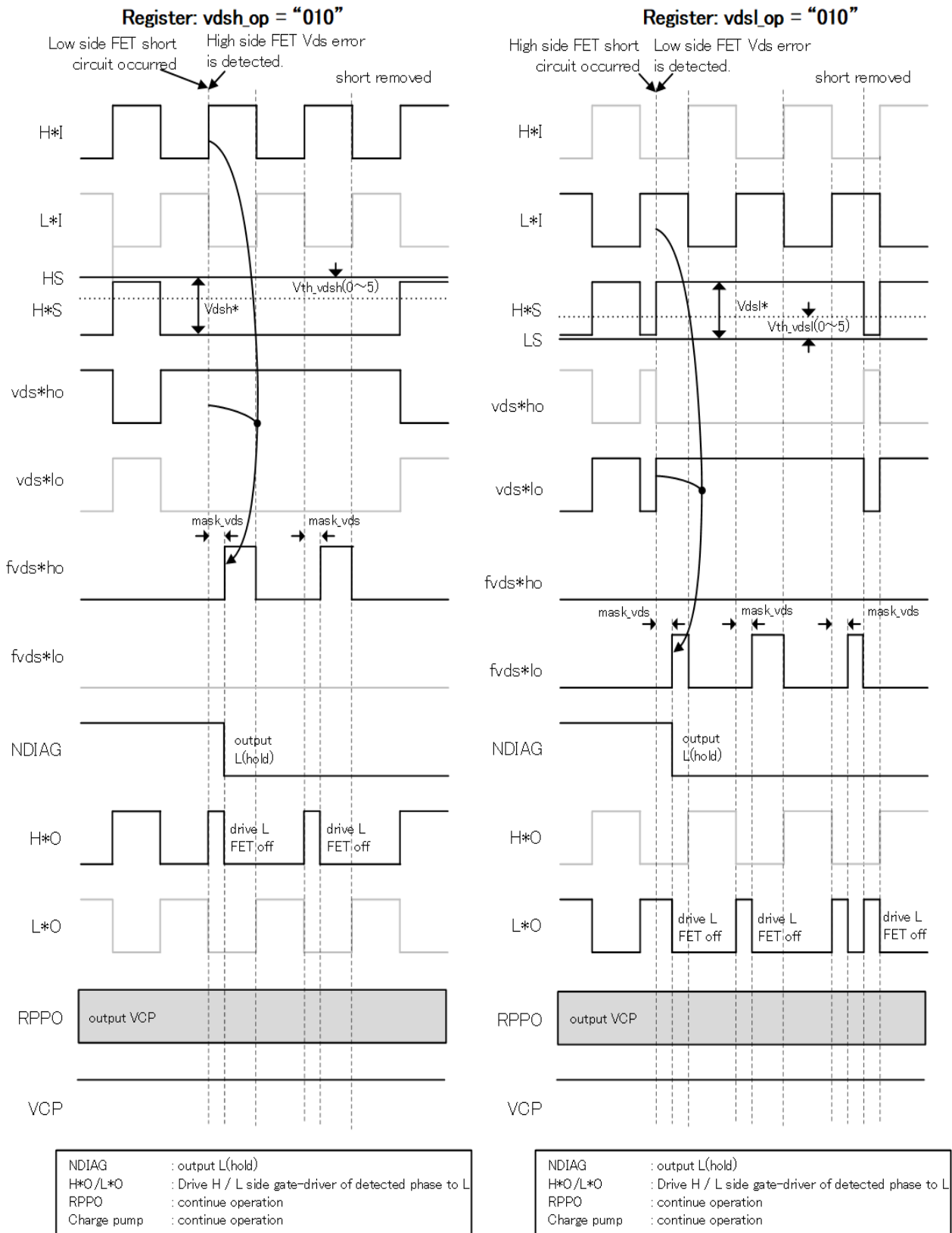
Fig. 7.6.7.4 Short-Circuit Detection Timing Chart (In the case of register: vds l _op = vds h _op "010")
