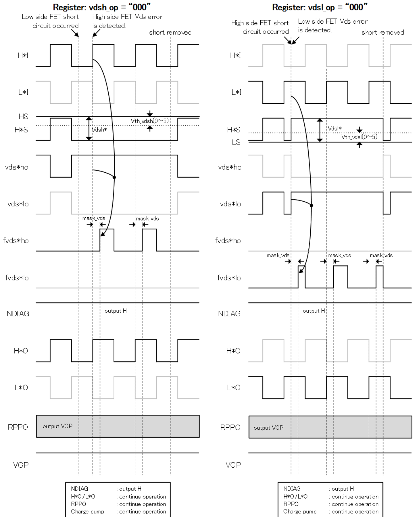
Fig. 7.6.7.2 Short-Circuit Detection Timing Chart (In the case of register: vds l _op = vds h _op "000")
