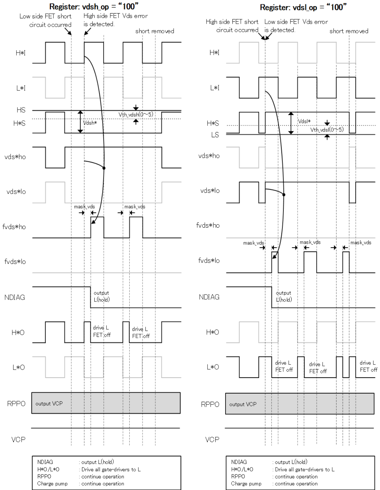
Fig. 7.6.7.6 Short-Circuit Detection Timing Chart (In the case of register: vds l _op = vds h _op "100")
