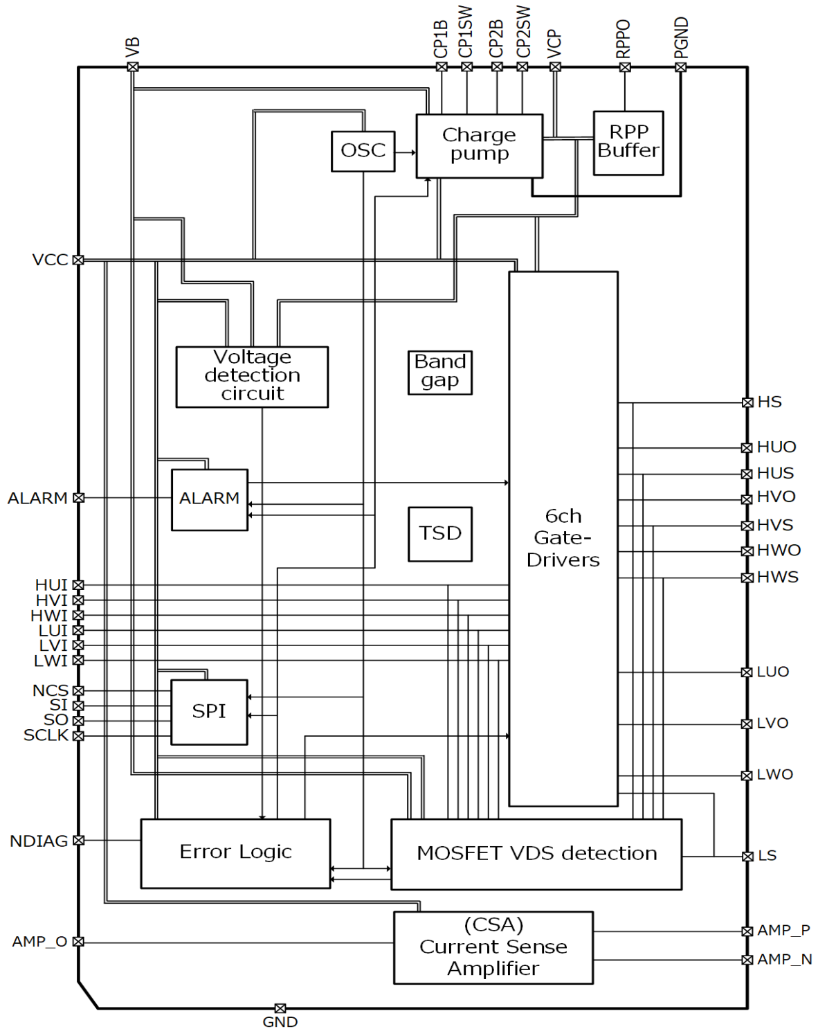
Fig. 4.1 Block Diagram
