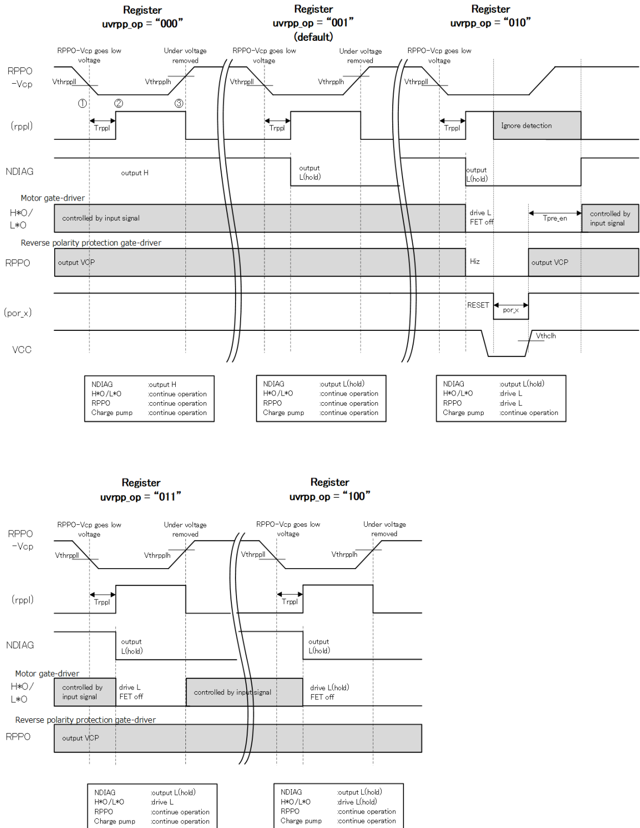
Fig. 7.6.3.2 RPP0 Under Voltage Detection Timing Chart
