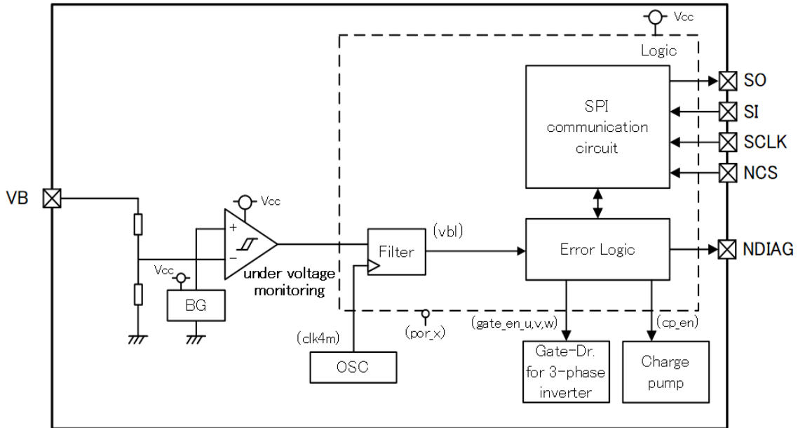
Fig. 7.6.2.1 VB Under Voltage Detection Block Diagram
