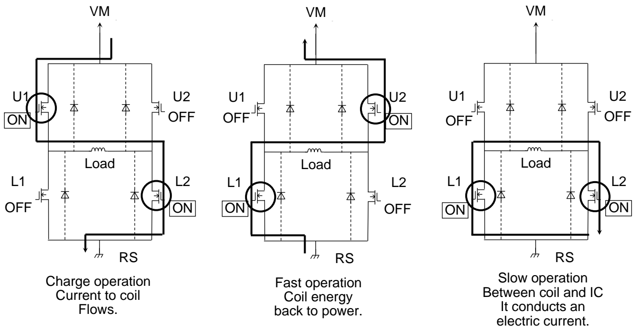
Figure 7.6 Output Stage Transistor Operating Mode
