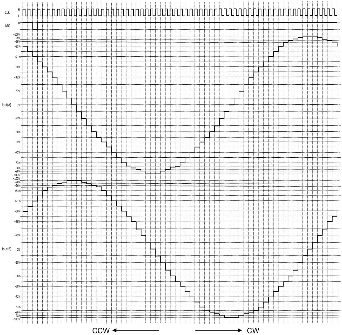
Figure 7.1.7.6 1 / 16 step Setting
