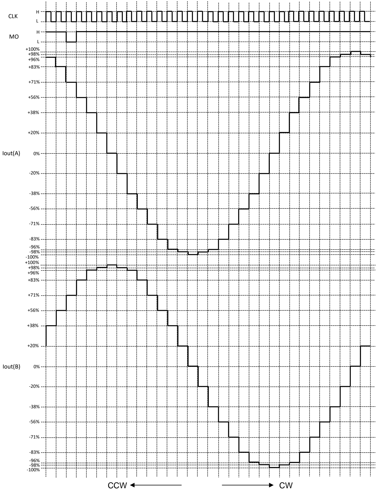
Figure 7.1.7.5 1 / 8 step setting
