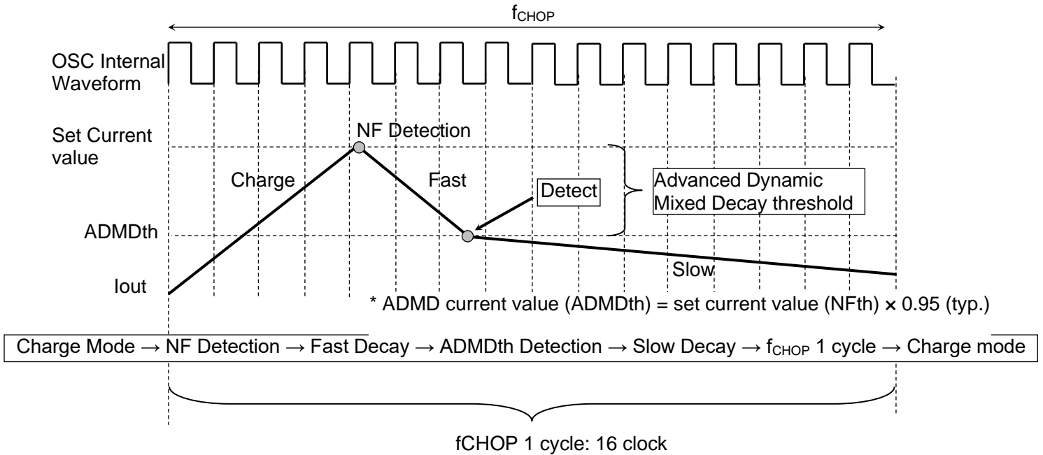
Figure 7.1.9.3.1 Advanced Dynamic Mixed Decay Constant Current Control
