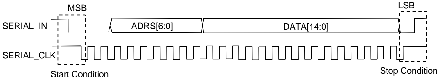
Figure 7.5 Serial Format
