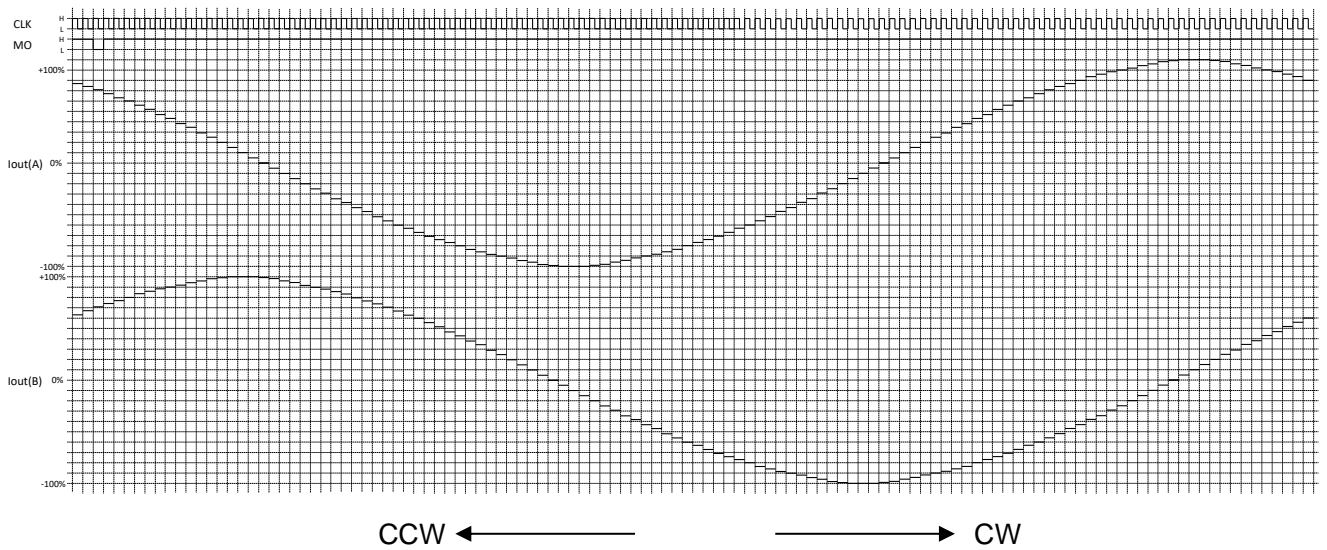
Figure 7.1.7.7 1 / 32 step Setting
