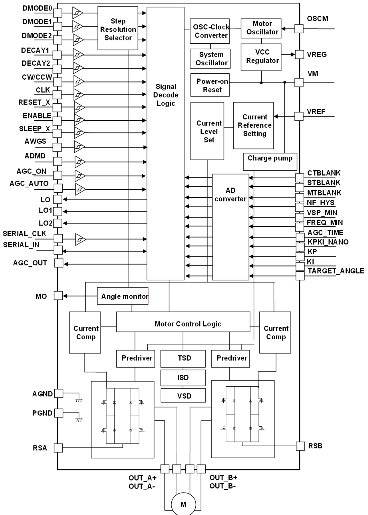
Figure 3 Block diagram
