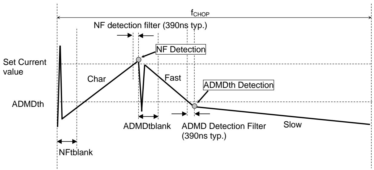
Figure 7.1.9.3.2 Advanced Dynamic Mixed Decay Constant Current Control
