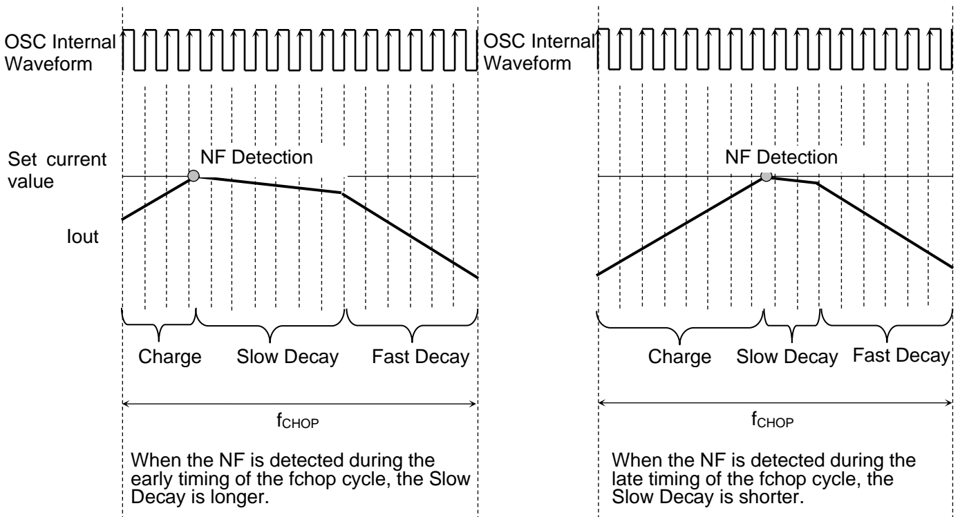
Figure 7.1.9.2.1 Constant Current PWM Operation Time
