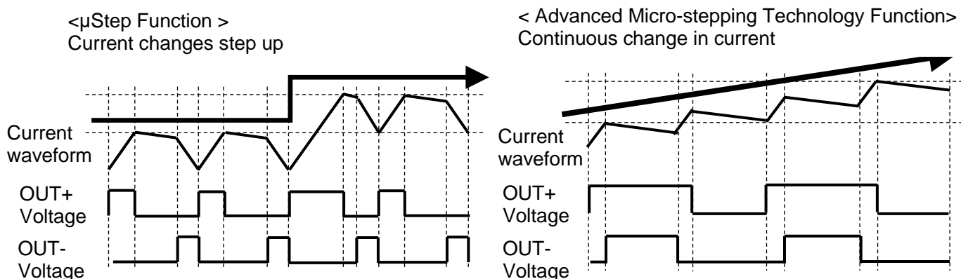
Figure 7.4.1 μStep and Continuous Micro-stepping
