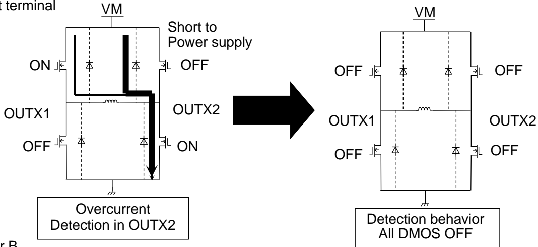
Figure 7.6.5.2.2 When an overcurrent is detected in the DMOS section (1)
