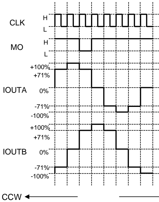
Figure 7.1.7.3 Half step (b) setting
