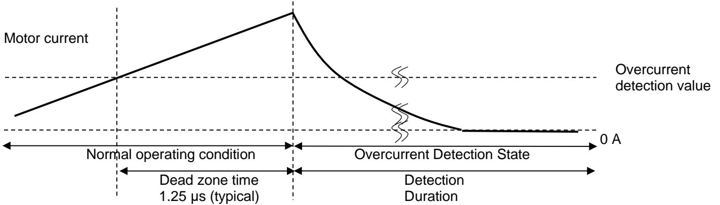
Figure 7.6.5.2.1 Overcurrent Detection
