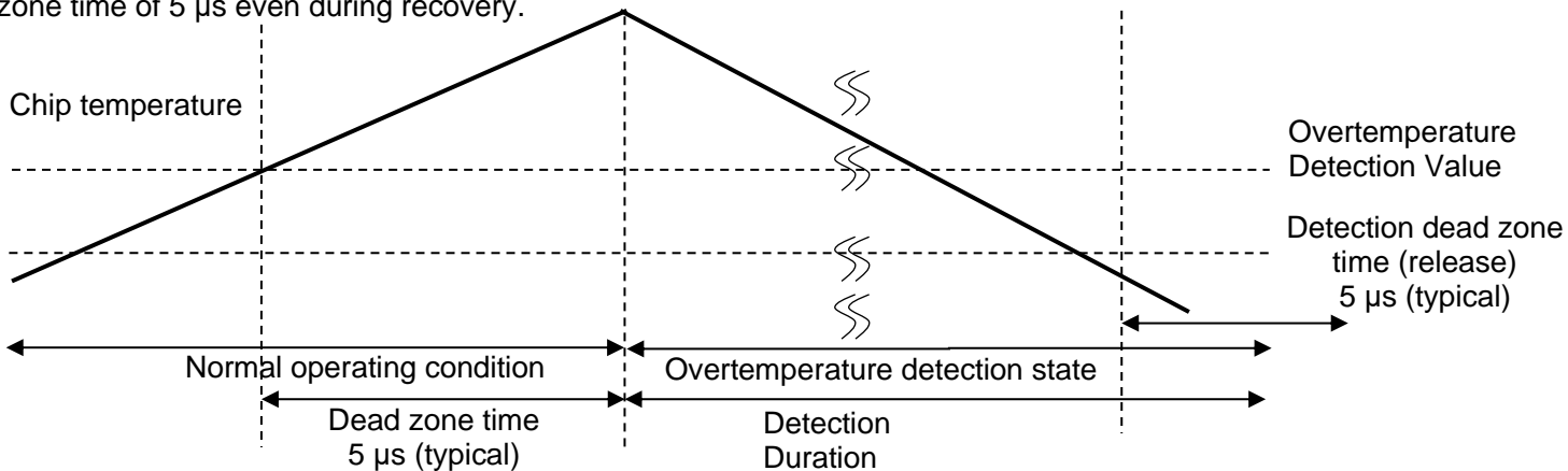
Figure 7.6.5.1.1 Overtemperature Detection
