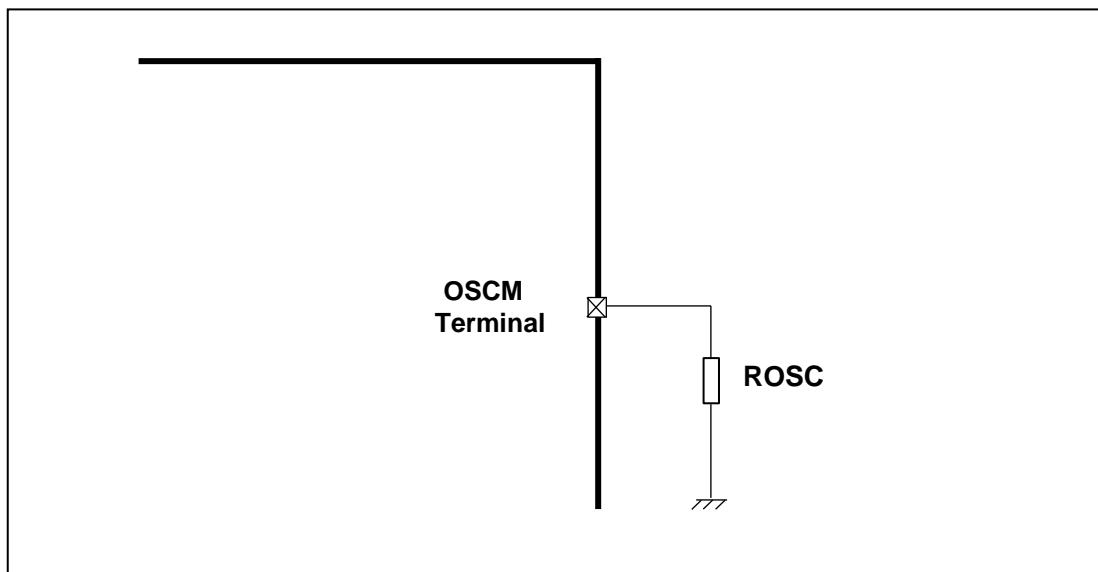
Figure 7.6.3 OSCM pin equivalent circuit
