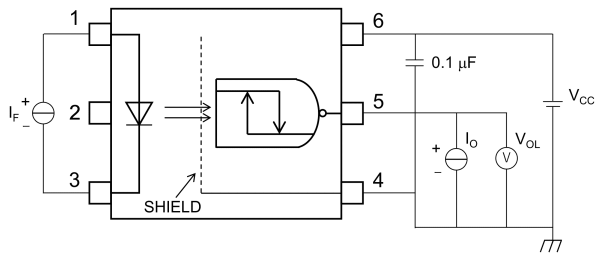
Fig. 13.1.1 V_{OL} Test Circuit
