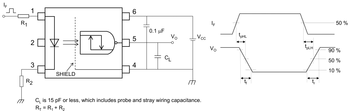
Fig. 13.1.5 Switching Time Test Circuit and Waveform
