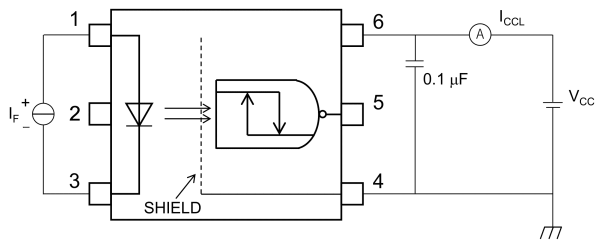
Fig. 13.1.3 I_{CCL} Test Circuit
