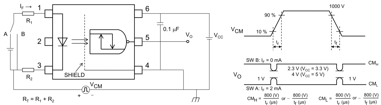
Fig. 13.1.6 Common-Mode Transient Immunity Test Circuit and Waveform
