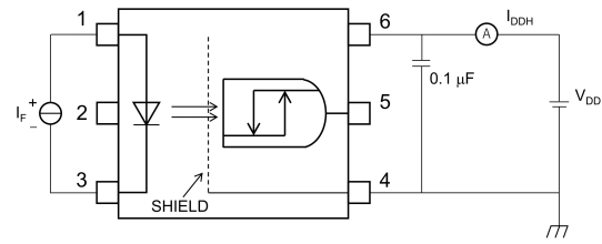
Fig. 13.1.4 I_{DDH} Test Circuit
