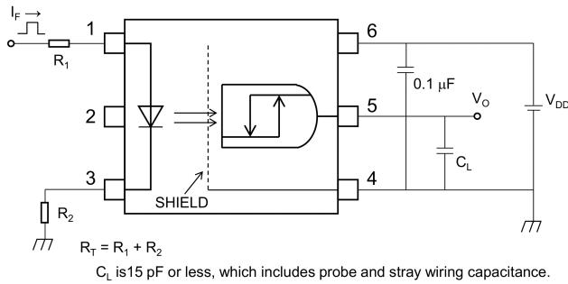
Fig. 13.1.5 Switching Time Test Circuit and Waveform
