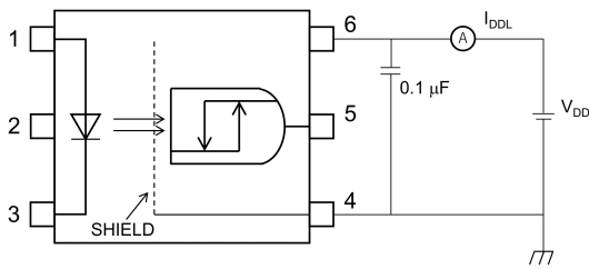
Fig. 13.1.3 I_{DDL} Test Circuit
