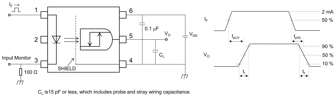
Fig. 13.1.6 Switching Time Test Circuit and Waveform
