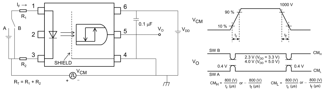
Fig. 13.1.7 Common-Mode Transient Immunity Test Circuit and Waveform
