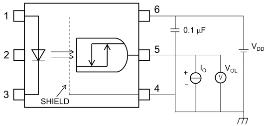
Fig. 13.1.1 V_{OL} Test Circuit
