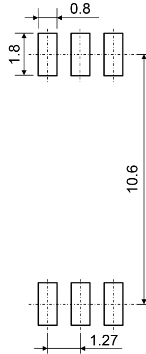
Fig. 15.1 Lead Forming Option (LF4)
