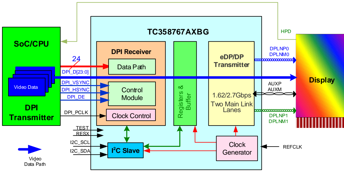
Figure 1.2 System Overview with TC358767AXBG in MODE_P21 Configuration
