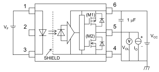
Fig. 13.1.2 I_{OPL} Test Circuit
