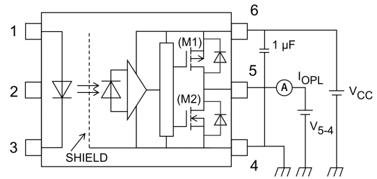
Fig. 13.1.2 I_{OPL} Test Circuit
